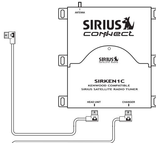
Optional Kenwood SIRIUS-READY Headunit (5L-Bus CD Player or Mobile Multimedia Station)
